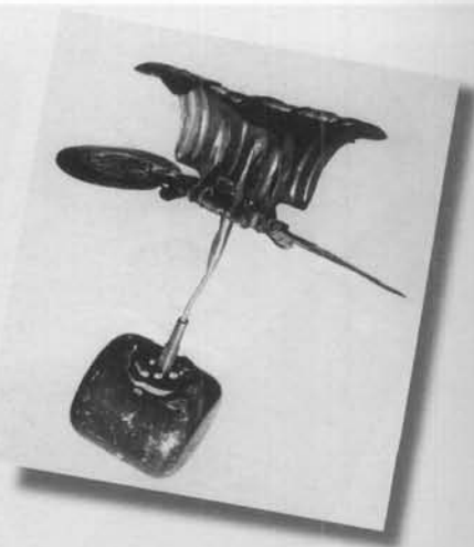
An SD-2 pictured in the open, live, condition in which it fell to earth slowed by the rotating 'wings'. For a time this weapon caused severe disruption to the lives of the citizens of Grimsby, following the Luftwaffe attack on the night of 13/14 June 1943.
