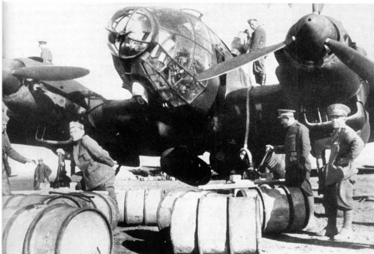
LEFT: Italian airmen at the airfield on Rhodes assist with the refuelling of an He 111 H-6 of KG 4. The aircraft is loaded with a pair of LMB mines, probably intended for the approaches to Alexandria harbour or the Suez Canal.
