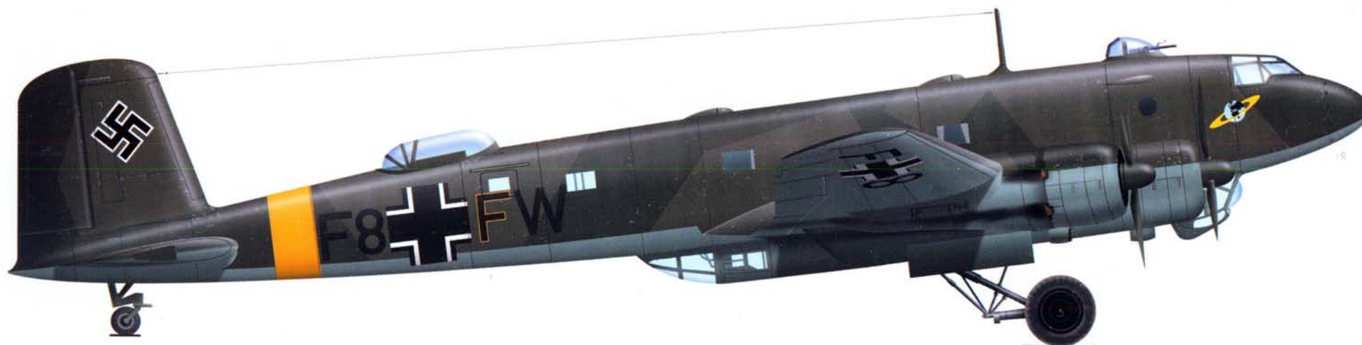
Focke-Wulf Fw 200 C-3 of 12.(Erg)/KG 40 based at Chateaudun in France between late 1942 and February 1944 The aircraft has the standard naval uppersurface camouflage of two dark greens (RLM 72 and 73) with pale blue (RLM 65) beneath. The unusual style of Balkenkreuz on the fuselage sides was quite common to Fw 200s for some reason. The Geschwader's famous 'world in a ring' badge was painted on the nose.
