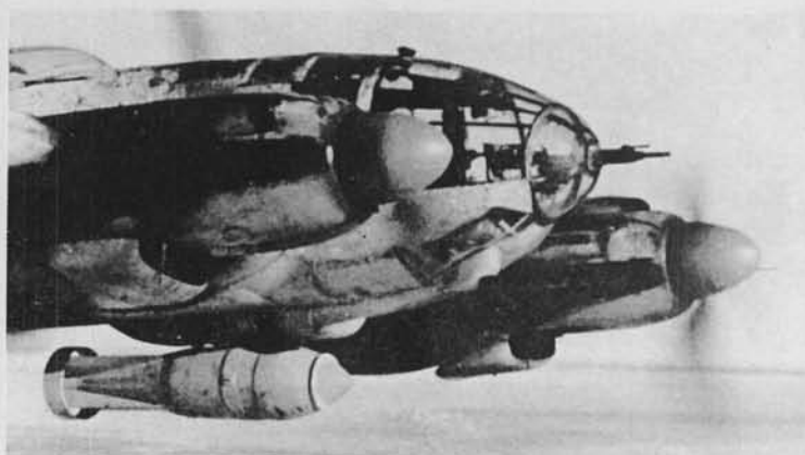
ABOVE: An He 111 of an unidentified unit on its way to attack a target over the Eastern Front. It carries a single SC 1000 (2,200 lb) bomb on the under-fuselage rack. On this type all weapons larger than an SC 250 (550 lb) bomb had to be carried externally.
