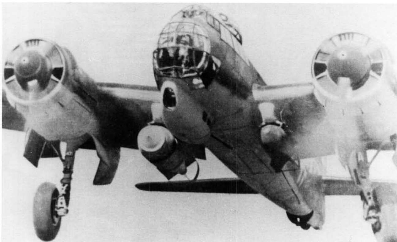
LEFT: A Ju 88 pictured immediately after take-off for an attack mission. The port undercarriage unit is in the process of retracting and has started to turn through 90 degrees so the wheel can lie flat in the nacelle. The retraction of the tail wheel is almost complete. The aircraft carries an SC 1000 bomb on the starboard side and an SC 250 on the port side, and its outer bomb carriers have been removed.
