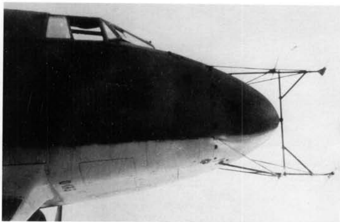
ABOVE: The nose-mounted transmitter aerials of the Rostock radar fitted to an Fw 200.
