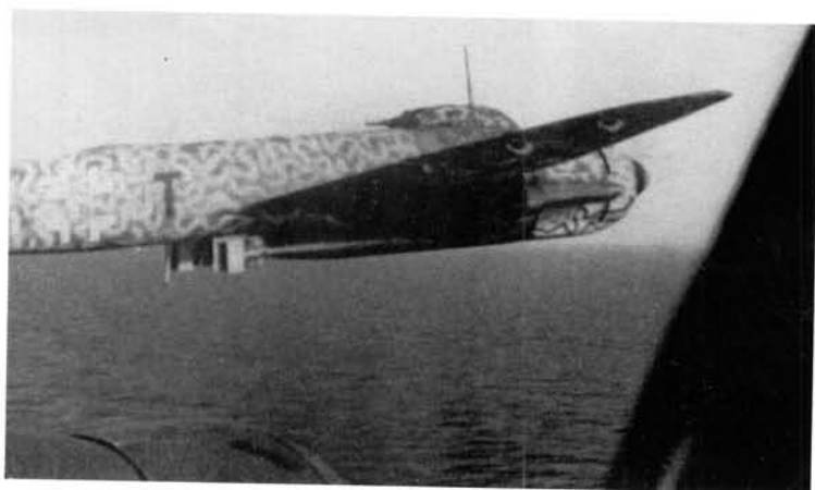
ABOVE: This Ju 88 coded 3Z+UT from 9./KG 77 is flying at low level above the water loaded with two torpedoes
