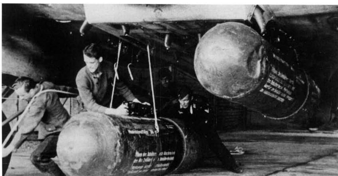
LEFT: Armourers loading LMB 1000 kg parachute mines on the fuselage racks of a He 111. In addition to their intended role of rendering waterways hazardous for shipping, these thin cased weapons were often fitted with impact fuses and employed against land targets.
