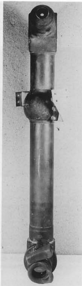
ABOVE: The rear-view gunsight as used with the R23 field modification kit, salvaged from a crashed Do 217 shown below.
