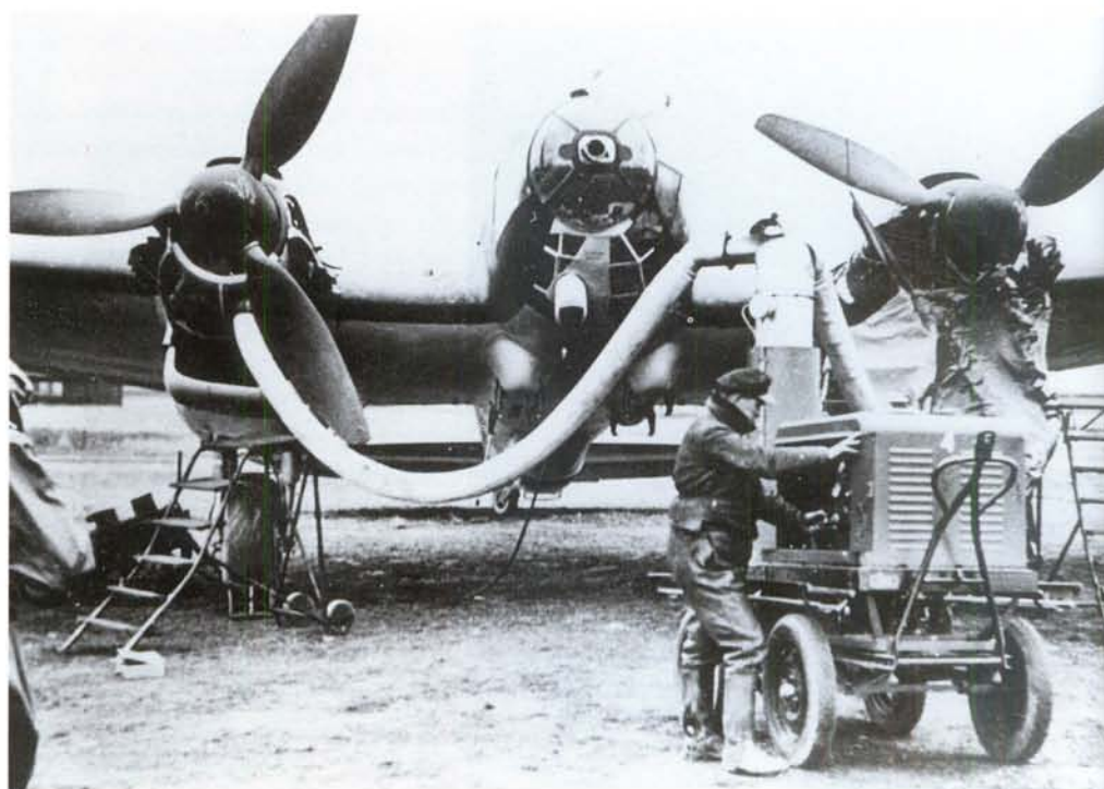
LEFT: A combustion heater used to warm the engines' coolant and lubrication systems of a He 111 before starting the engine. This was a particularly important item of equipment for units operating on the Eastern Front during the winter months.
