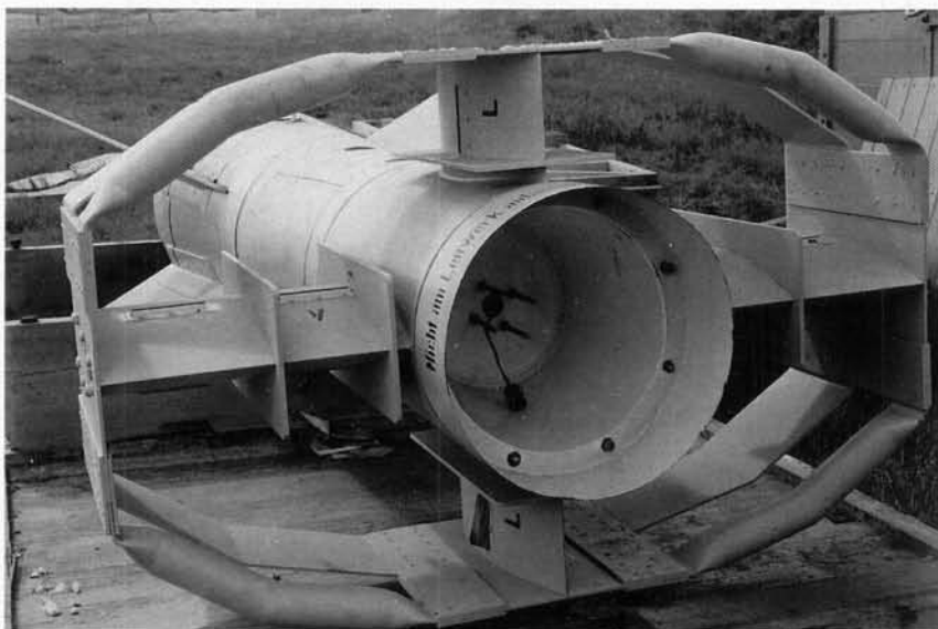
LEFT AND BELOW: Two photographs of a Fritz-X (PC 1400 FX) radio-controlled bomb on its delivery stand.
