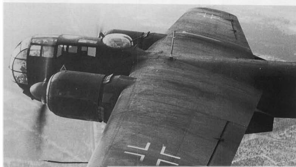
ABOVE: A close-up of a Do 217 K of KG 2 in flight over France taken from another aircraft in the formation.
