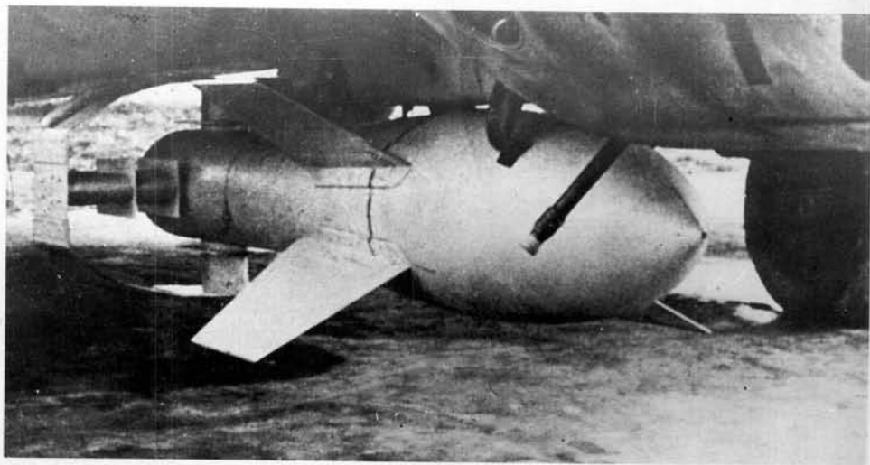
ABOVE: The Fritz-X radio-guided armour-piercing bomb, weighing 1,400 kg (3,090 lbs), pictured mounted on the fuselage bomb rack of a He 177. Released from altitudes around 6,100 metres (20,000 ft), the unpowered weapon achieved an impact velocity close to the speed of sound, enabling it to penetrate the deck armour of a heavy cruiser or a battleship.
