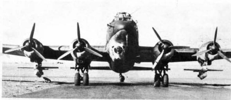
ABOVE: An Fw 200, possibly at the Erprobungsstelle Karlshagen, fitted with an experimental installation of one Hs 293 mounted under each outer engine. It is not thought that the aircraft was ever sent into action in this configuration.
